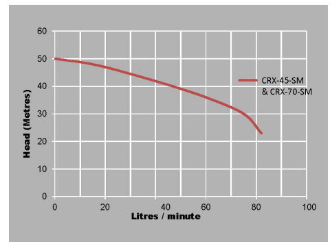
Submersible Pump Performance Curve
