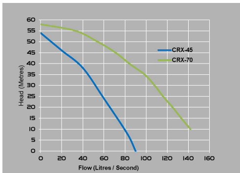
Horizontal Pump Performance Curve
